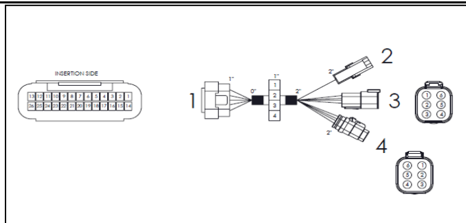
Picture 1. SA-R Harness
